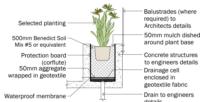
03 ON STRUCTURE PLANTER TYPICAL DETAIL All structures and grades to engineers details 1:50
