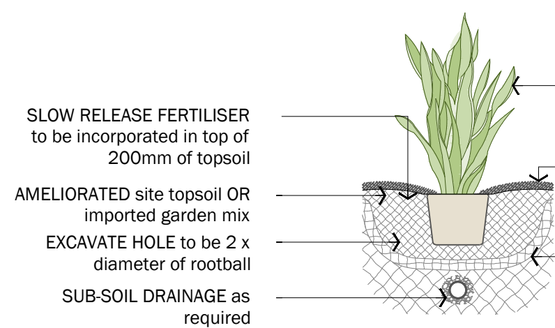
02 SHRUBS + PERENNIALS PLANTING DETAIL 1:50
