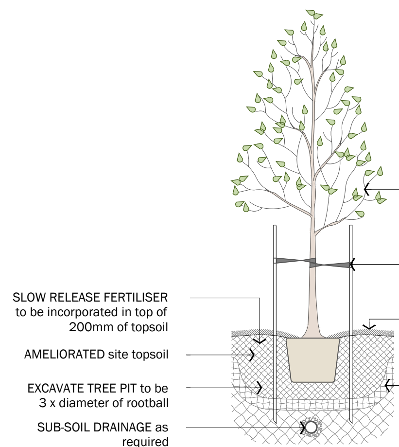
01 TREES PLANTING DETAIL 1:50
